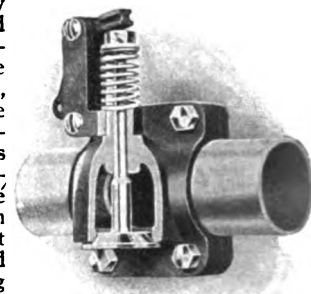
CLAMP VALVE FITTED TO PIPE.
